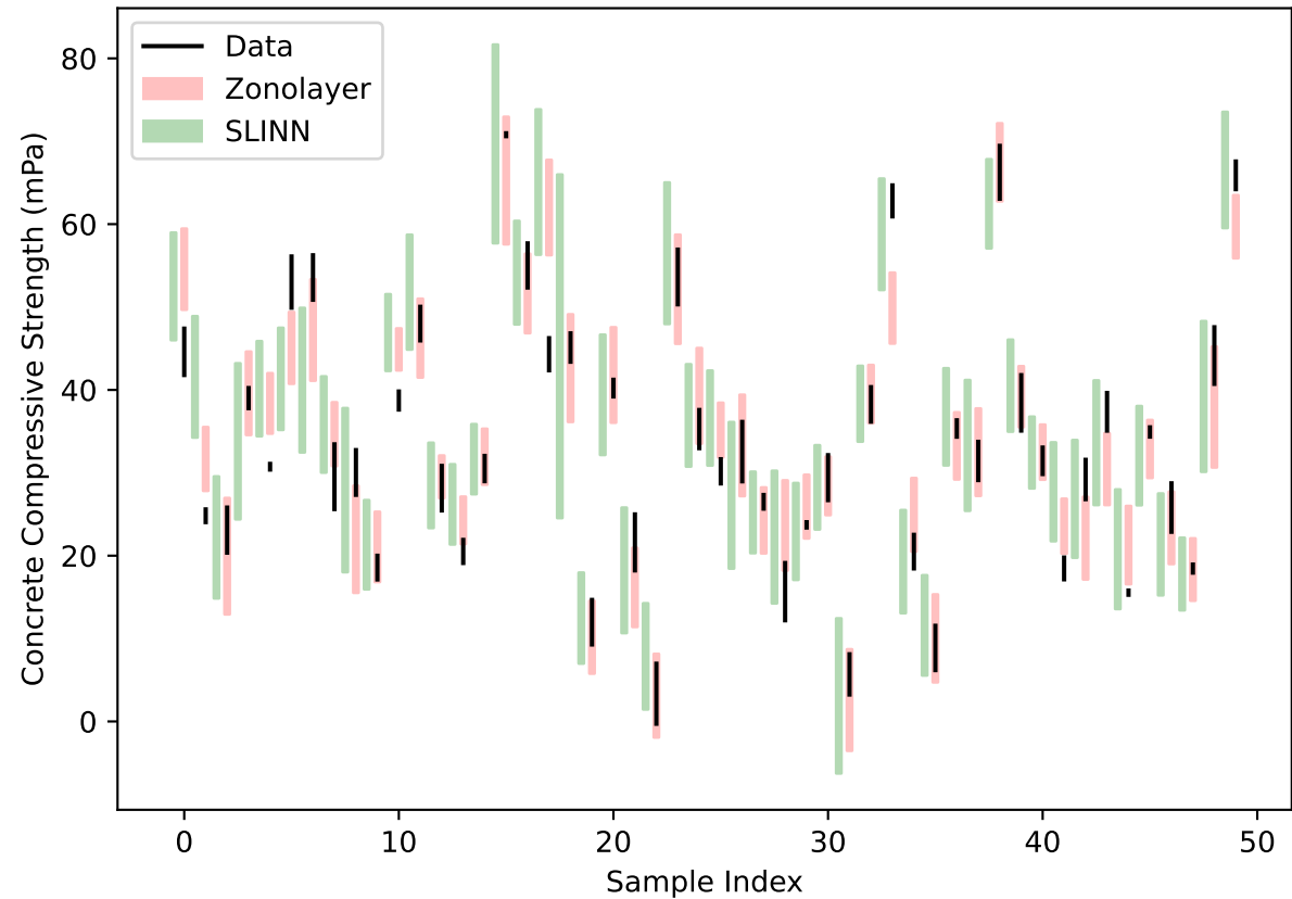
Concrete Compressive Strength Dataset
